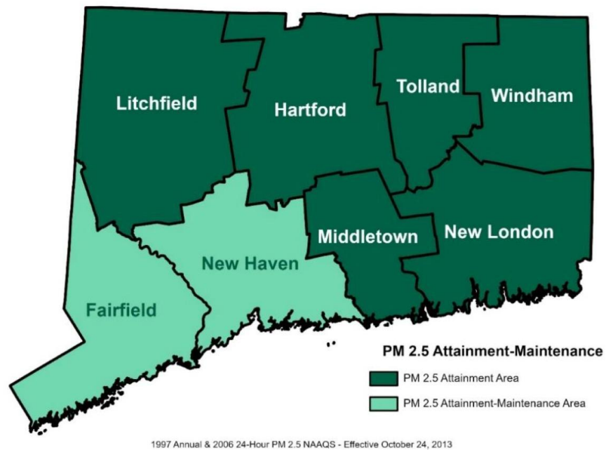
Figure 10. Connecticut PM2.5 Attainment/Maintenance Area
